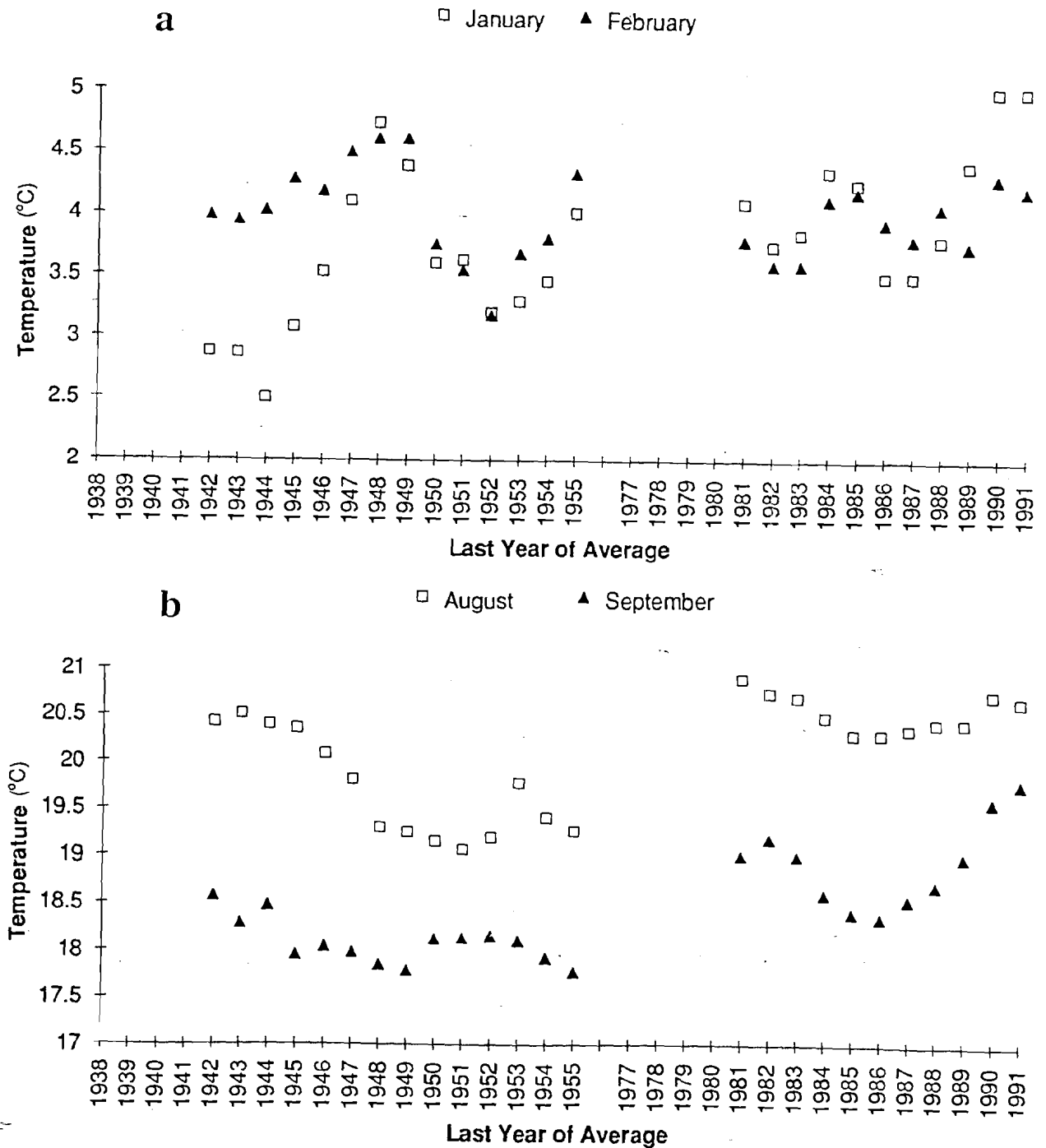
Figure 7.--Five year averages of mean monthly water temperature at Bonneville Dam/Warrendale during annual minimum temperatures (January and February) (a) and annual maximum temperatures (August and September) (b) for water years 1938-91. Data for 1956-76 were not available. The year given for each data point is the last year computed in the average. Data from Sylvester (1958), USGS (1978b-92b).
