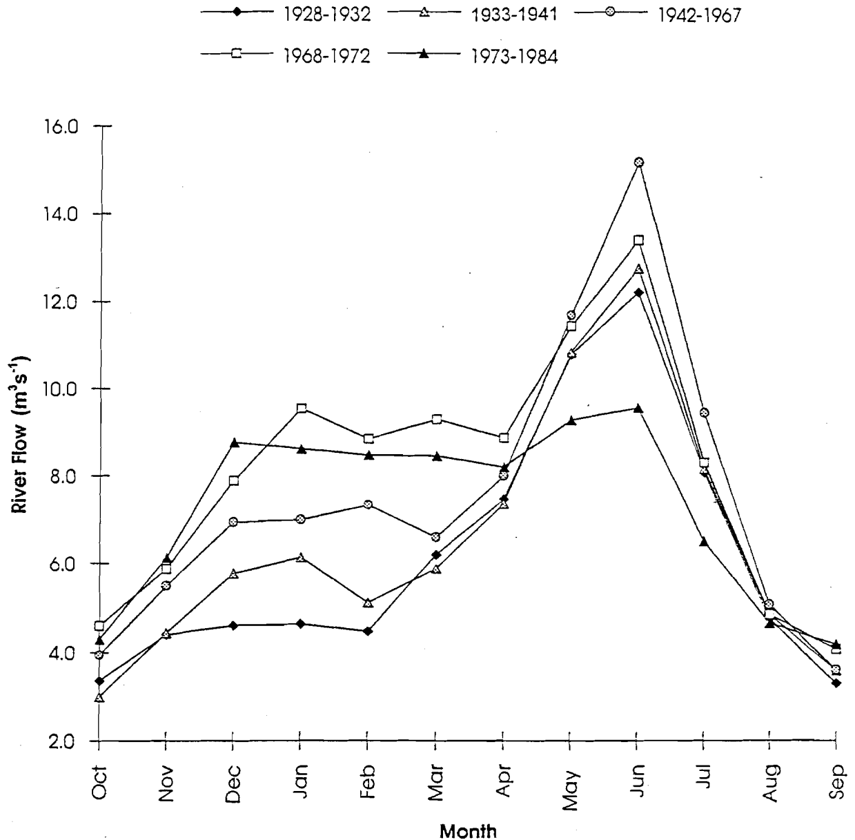
Figure 4.--Mean monthly flow at the mouth of the Columbia River 1928-84, divided into five time periods to reflect the increasing active storage capacity of Columbia and lower Snake River reservoirs. The active storage and dams completed for each period are as follows: 1928-1932--no active storage or dams on the Columbia River mainstem or lower Snake River; 1933-1941--less than 0.2 km 3 active storage; Rock Island (1933) and Bonneville (1938) Dams completed; 1942-1967--6.6-8.7 km 3 active storage; Grand Coulee (1942), McNary (1953), The Dalles (1957), Chief Joseph (1958), Brownlee (1959), Priest Rapids (1961), Oxbow (1961), Ice Harbor (1961), Rock Reach (1962), Wanapum (1964), and Wells (1967) Dams completed; 1968-1972--17.6-20.2 km 3 storage; Hugh Keenleyside (1968), Lower Monumental (1969), Little Goose (1970), and Dworshak (1971) Dams completed; 1973-1984--35.0-42.0 km 3 storage; Mica (1973), Lower Granite (1975), and Revelstoke (1983) Dams completed. Data from Orem (1968), USGS (1973-77, 1978a-85a).
