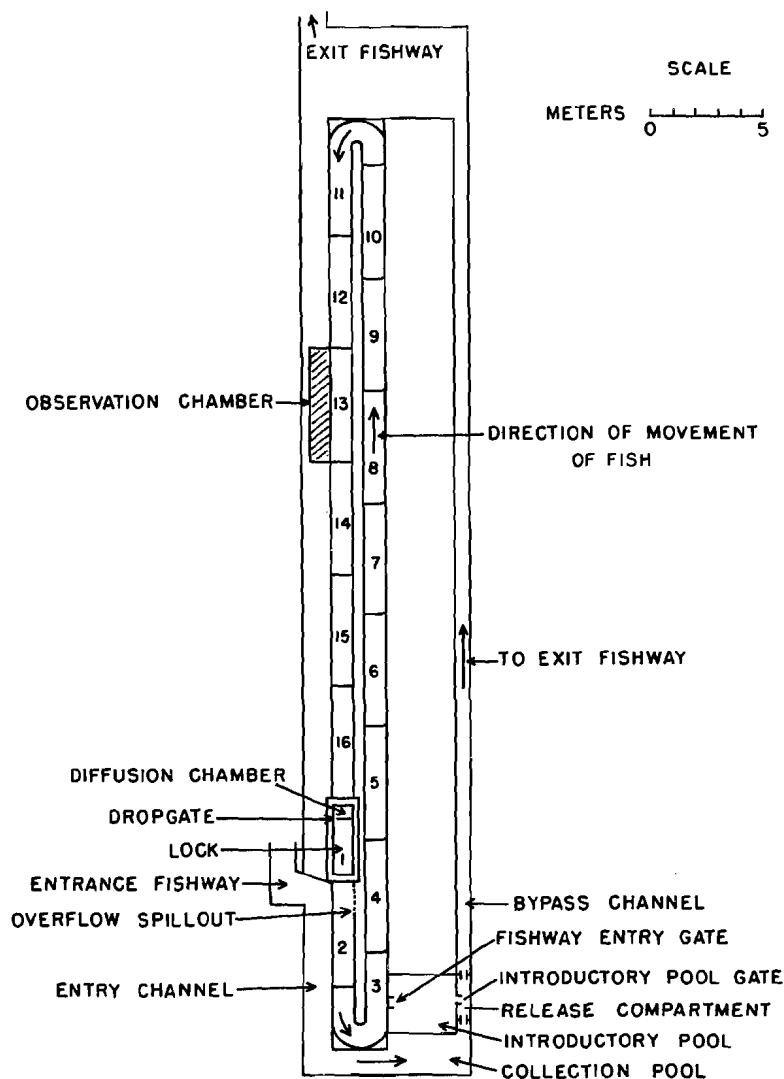
Figure 2.--Plan view of the 1-on-16 slope endless fishway with auxiliary approach channels and pools.
