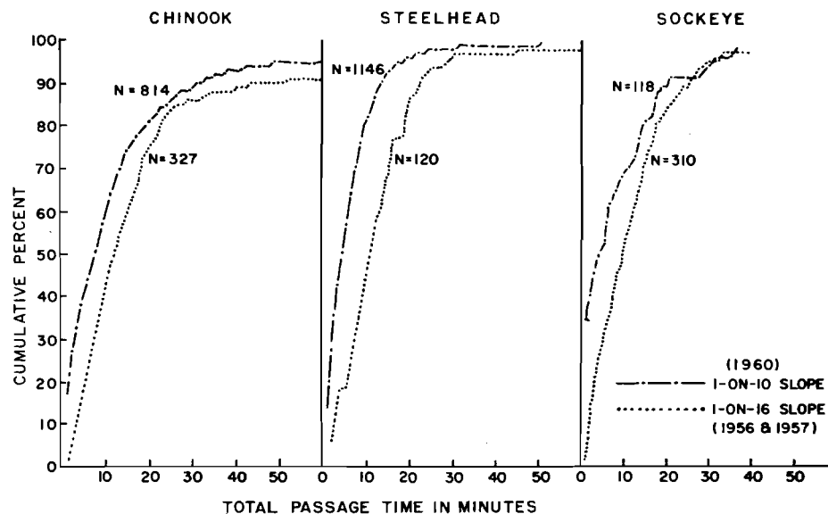
Figure 18.--Cumulative distribution of passage times of individual chinook, steelhead, and sockeye in 1-on-10- and 1-on-16-slope fishways. Number of fish completing a six-pool ascent by 1-minute intervals expressed as a cumulative percentage of total tested (1-on-10 slope--1960, 1-on-16 slope--1956 and 1957).
