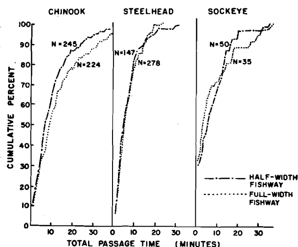
Figure 14.--Comparison of ascents of individual salmonids in the full-width and half-width fishway (test condition 1, table 1). Number of fish completing the ascent by 1-minute intervals expressed as a cumulative percent of total tested, June 8 to September 14, 1960.
