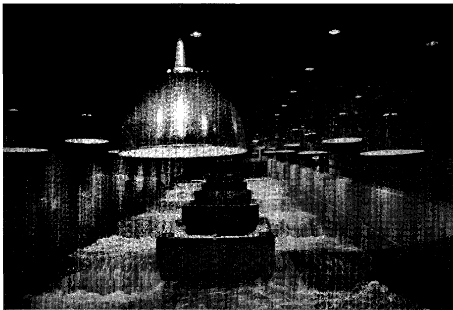
Figure 13.--The six-pool full-width test section of the Ice Harbor fishway design under proposed operating conditions.
