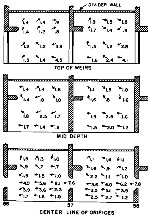
Figure 6.--Velocities (f.p.s.) and direction of flow in pools 57 and 58 during normal operation (test condition 1).
