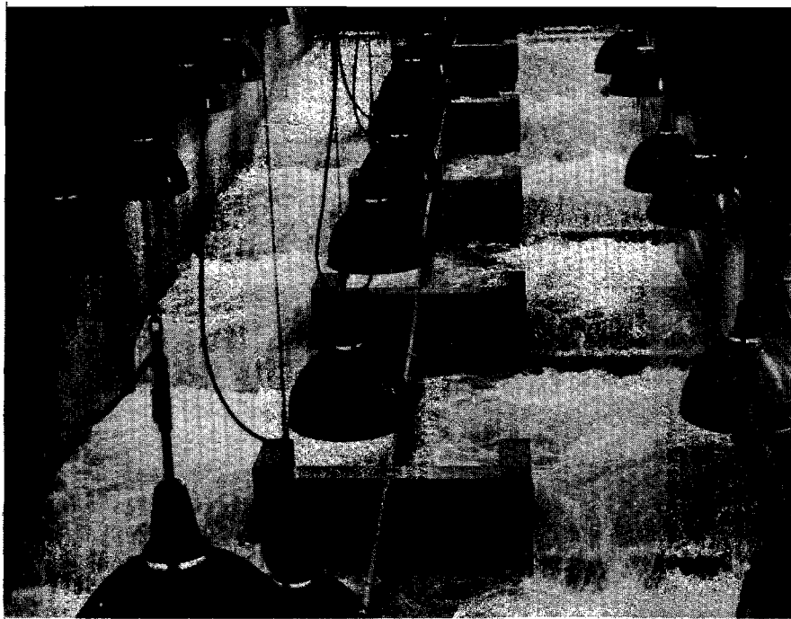
Figure 15.--Operational view of the Ice Harbor fishway with McNary crests on right and The Dalles crests on left. Note reduced turbulence in flow pattern on right. Corners on downstream face of the weir baffles on left are chamfered and those on right squared. Eventual design of prototype was modified to conform with structure on right.
