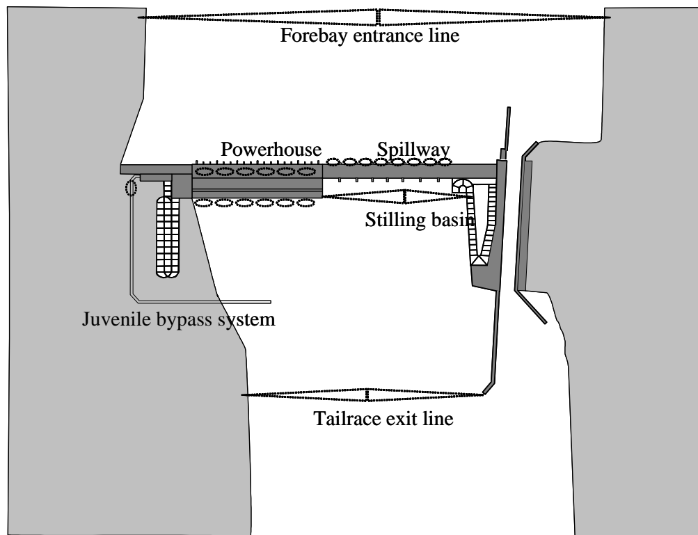
Figure 2. Lower Monumental Dam plan view showing approximate locations of detection zones for radiotelemetry receivers in 2006. Oval lines represent underwater antennas, and triangular lines represent aerial antennas.
