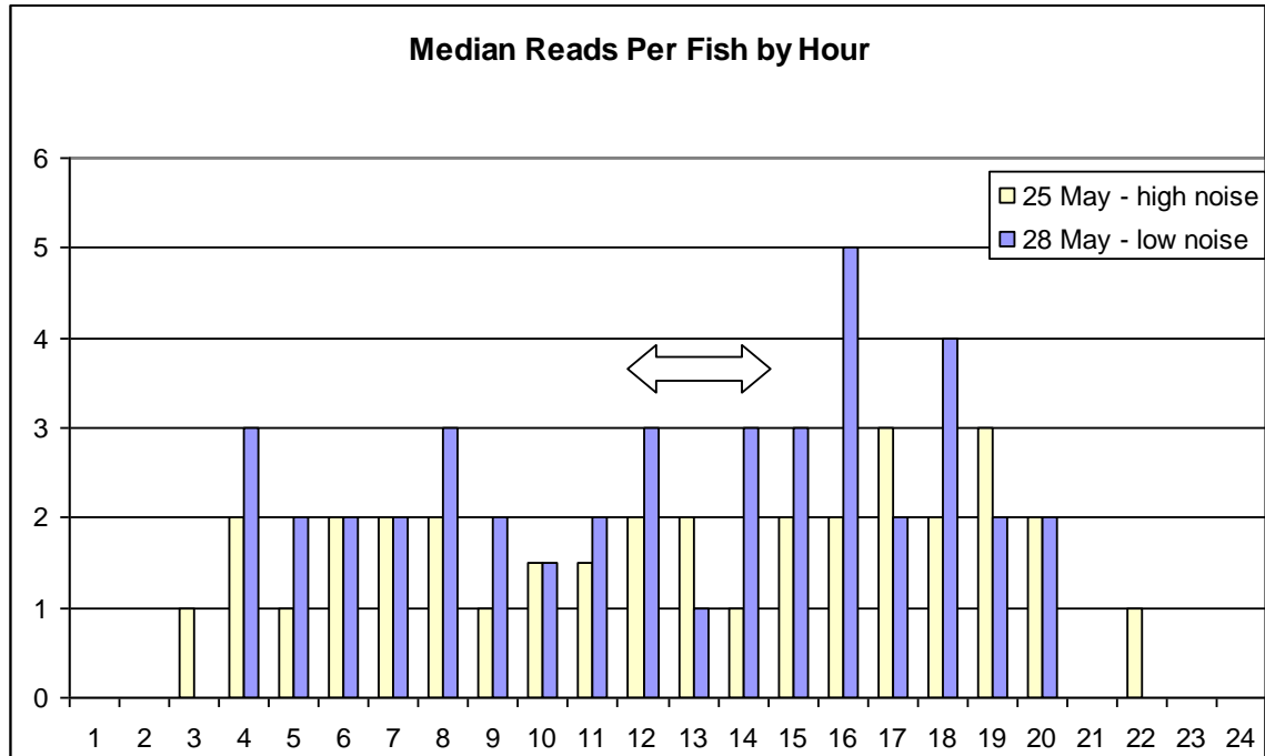
Appendix Figure 3. Median values of reads per ST-tagged fish on an hourly basis are presented for the noisiest day (25 May) and a typical low-noise day (28 May). The double-headed arrow denotes hours with the highest noise levels on 25 May.
