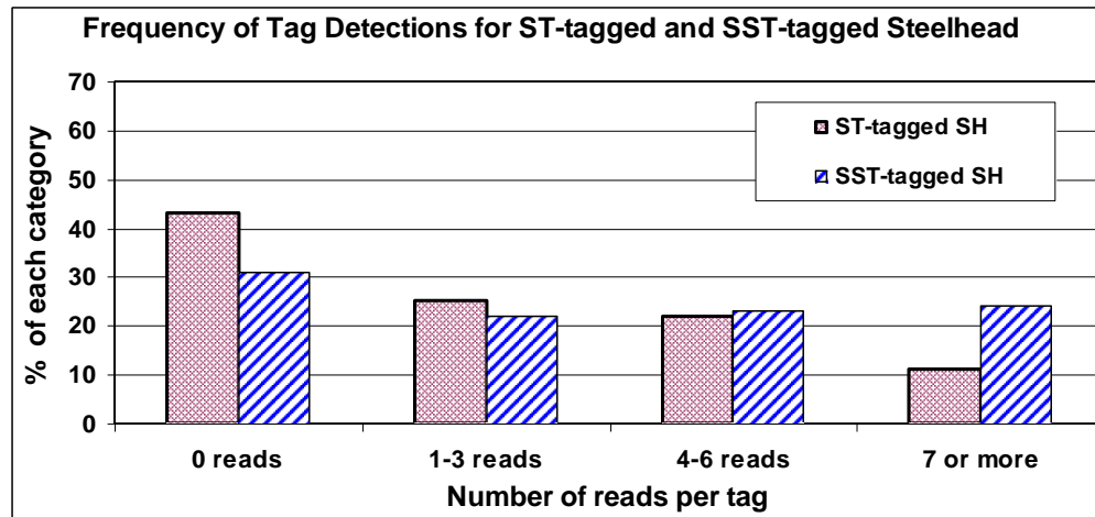
Figure 10. Detection frequency distributions for SST-tagged and ST-tagged steelhead released on 18-19 May 2006. Since we did not know how many fish had transited the flume, the 0-reads category was included.
