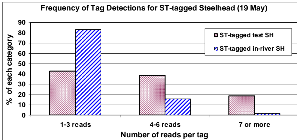
Figure 11. Frequency distributions for ST-tagged test steelhead (n = 40) and river-run steelhead (n = 218) detected on 19 May 2006. To show the patterns better, read-per-tag categories with similar values were combined. Since we did not know how many river-run fish had transited the flume, the 0-reads category was excluded.
