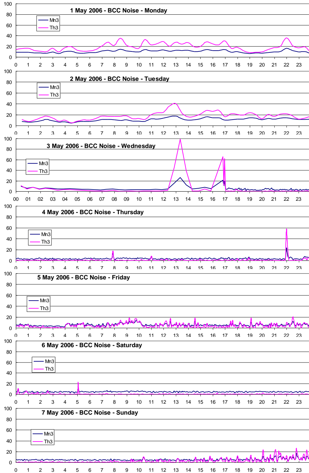
Appendix Figure 1. Hourly noise levels by day in the corner collector PIT-tag detection system (BCC) at Bonneville Dam measured by 1) medians of root mean square signal strength, as measured by DSP (Mn3) and 2) percentages of samples that exceeded threshold noise for tag-reading interference (Th3).
