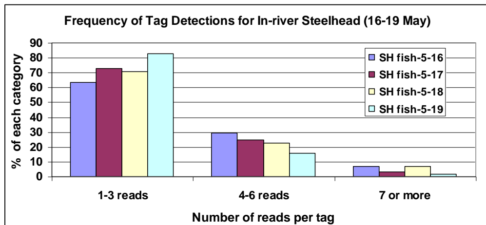
Figure 12. Frequency distributions for ST-tagged river-run steelhead detected on 16-19 May 2006 (numbers of fish detected ranged from 70 to 172). To show the patterns better, read-per-tag categories with similar values were combined. Since we did not know how many river-run fish had transited the flume, the 0-reads category was excluded.
