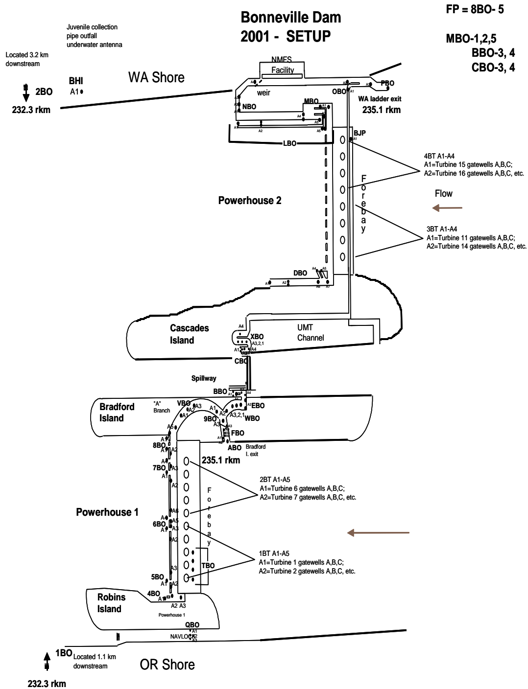
Bonneville Dam antenna setup.
