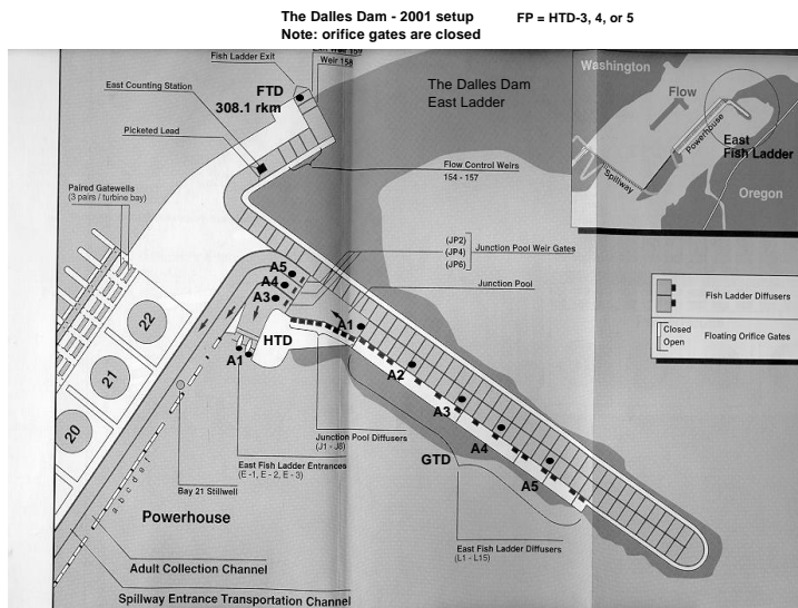
The Dalles Dam East Ladder
