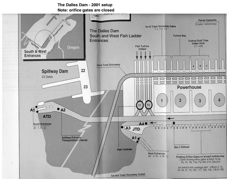
The Dalles Dam South and West Ladder Entrances
