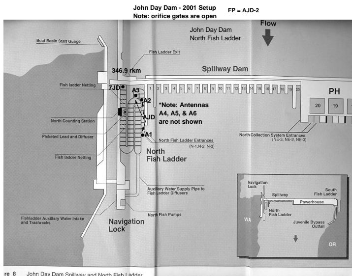
John Day Dam North Ladder
