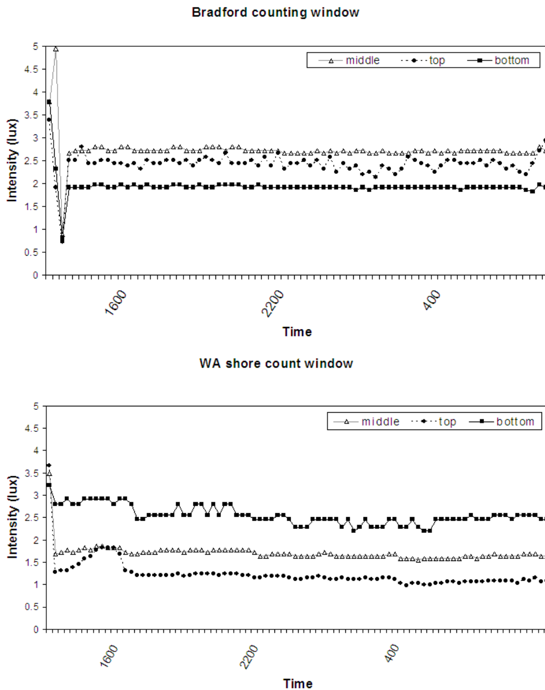
Figure 32. Light intensity (lux) recorded at positions in the middle and near the bottom and top of the count windows on Bradford Island (top) and the Washington shore (bottom).
