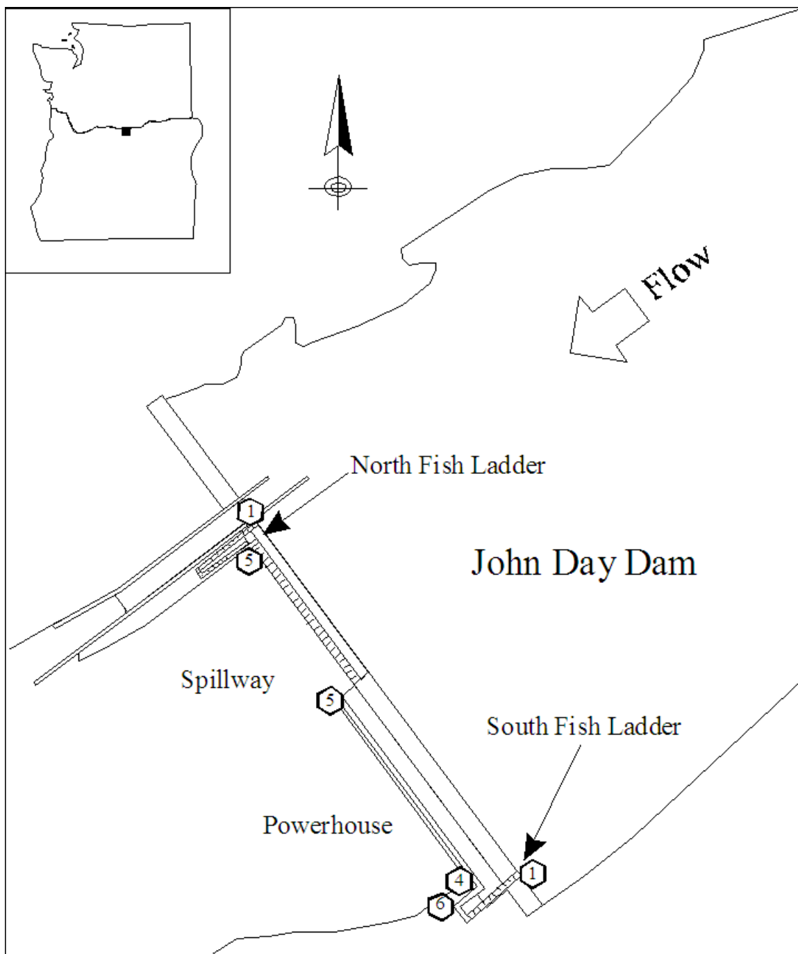
Figure 3. Study area at John Day Dam (solid square in insert). Receiver sites and the number of antennas at each receiver are denoted with hexagons.
