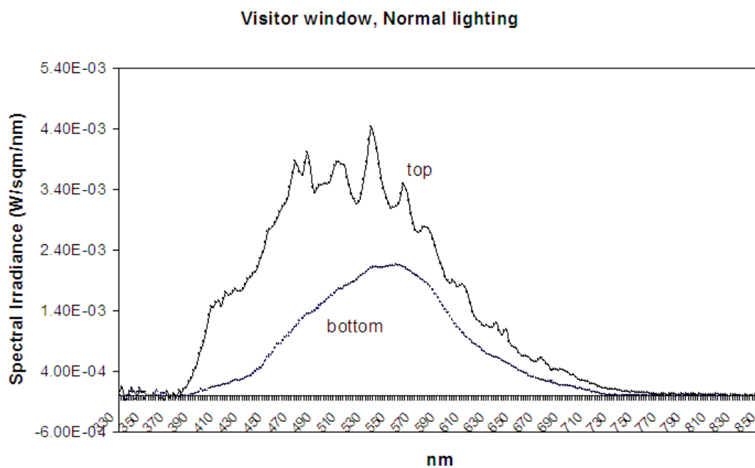
Figure 35. Spectral irradiance (W/sqm/nm) recorded near the top and bottom of the Bradford Island count (top) and visitor (bottom) windows during normal lighting conditions.
