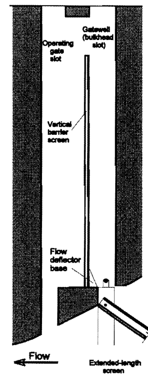
MBFVBS with flow deflector base
