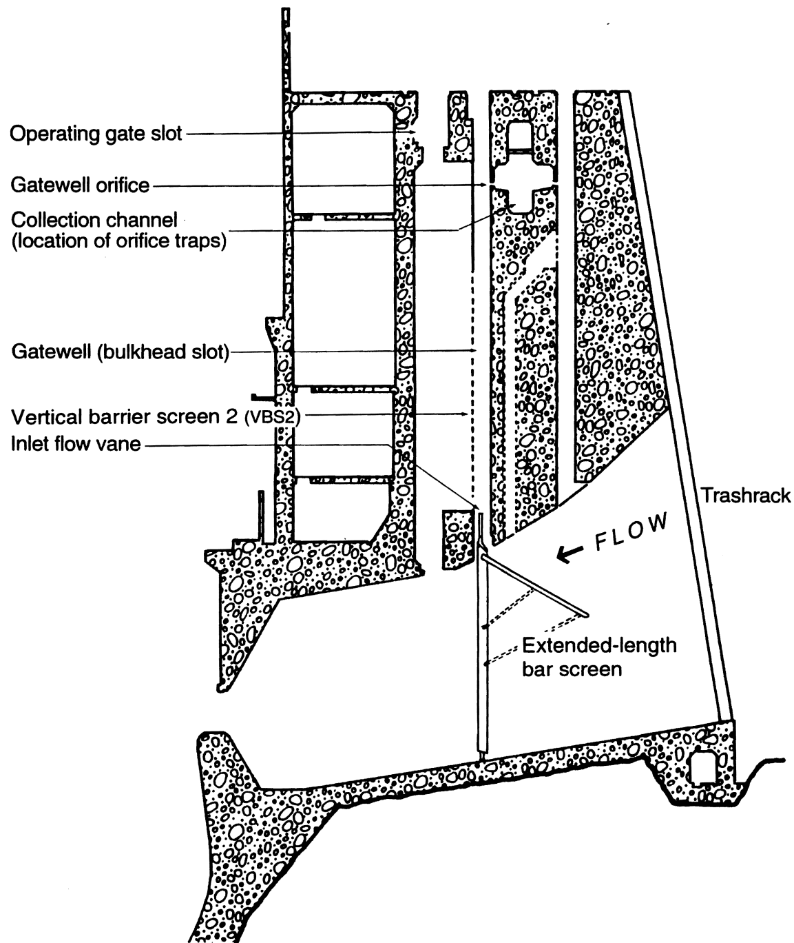
Figure 1. Cross section of turbine unit at Lower Granite Dam showing juvenile fish bypass system including extended-length bar screen, vertical barrier screen (VBS2), gatewell orifice, and collection channel. Also shown is location of orifice trap used in 1995 research.
