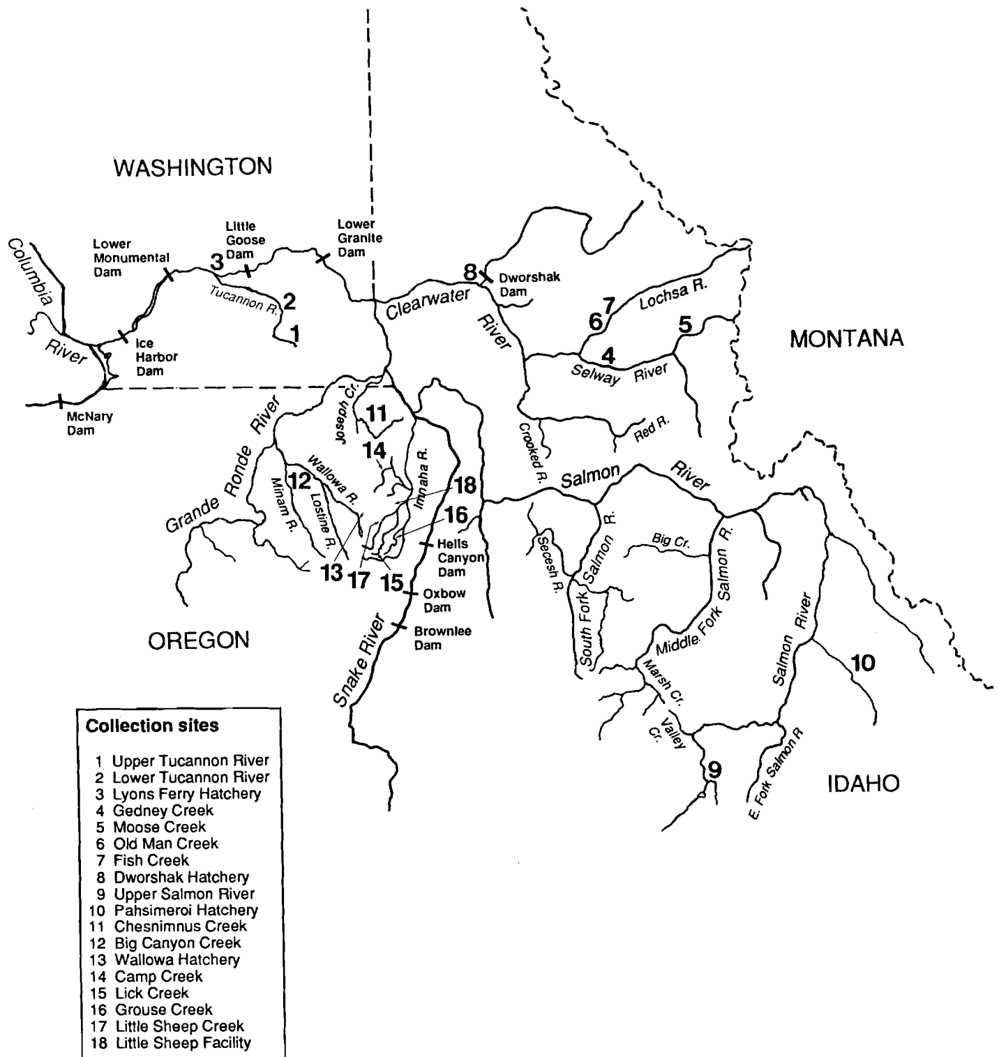
Figure 3.-- Map of study areas showing collection sites for steelhead samples.
