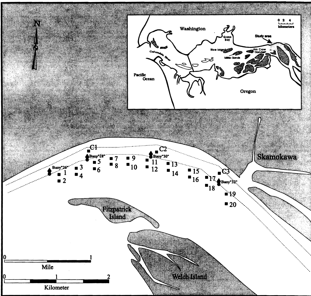
Figure 1. Locations of benthic invertebrate and sediment sampling stations in and adjacent to a proposed channel widening area (River Mile 31-34) in the Columbia River estuary. The North Transect stations (odd-numbered) were completely within the potential impact area, and the South Transect stations (even-numbered) were located along the southern boundary of the potential impact area or just south of the area. Stations C1-C3 were reference stations located in the navigational channel; the channel is indicated with dotted lines.
