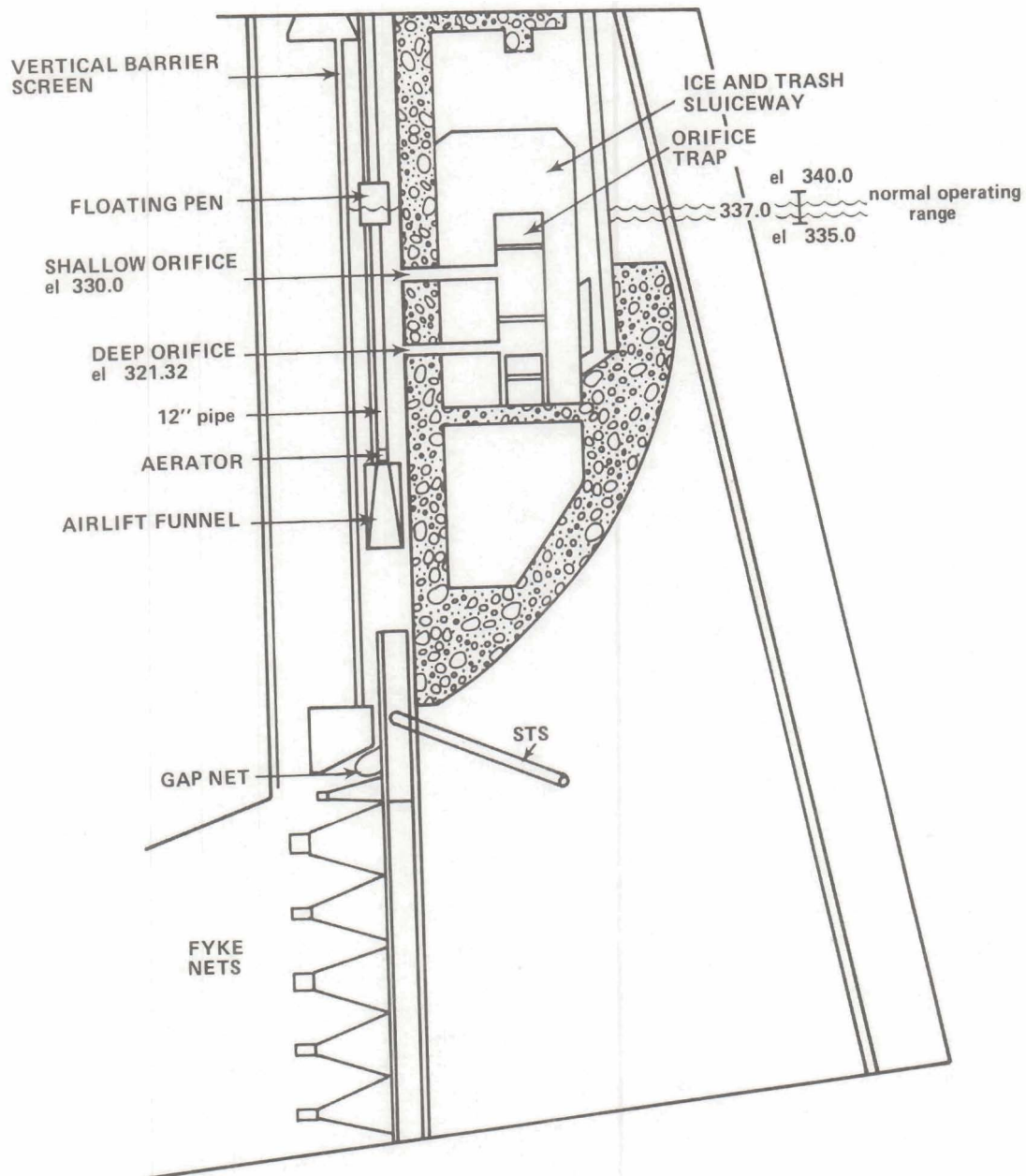
Figure 1.--Transverse section through Unit 6-B of McNary Dam showing experimental and handling equipment used for research in 1981.
